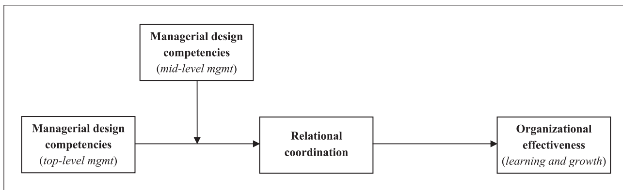
Figure 1. Research framework.
